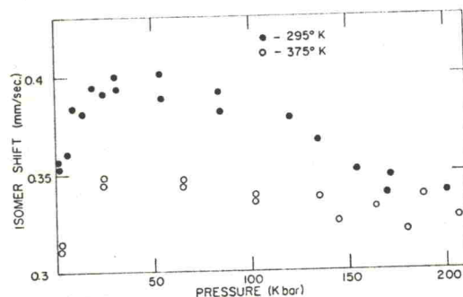
FIG. 3.—Isomer shift vs. pressure—ferric acetyl acetate (Fe(III)).
